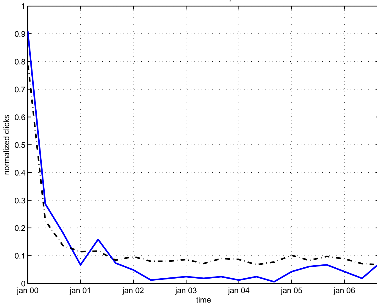
constraint duality
