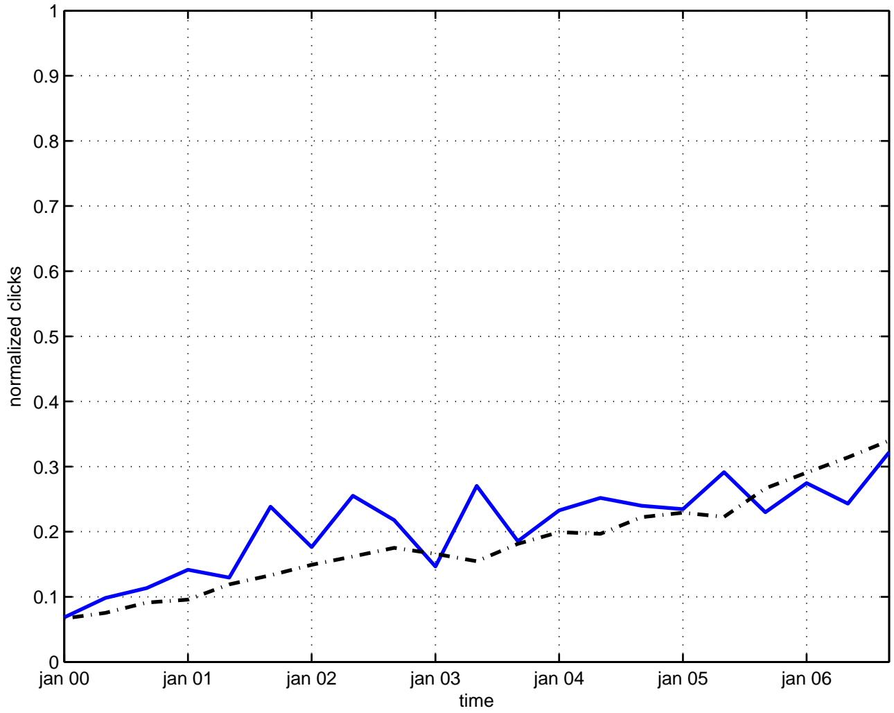
conservation law
