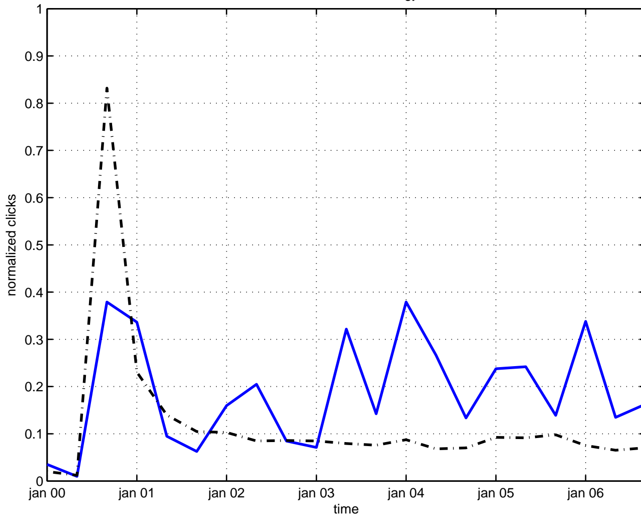
conservation law energy
