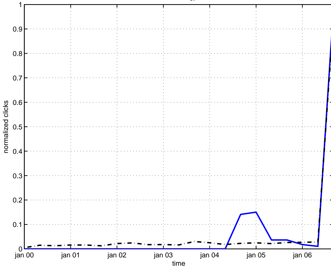
conservation law energy-momentum
