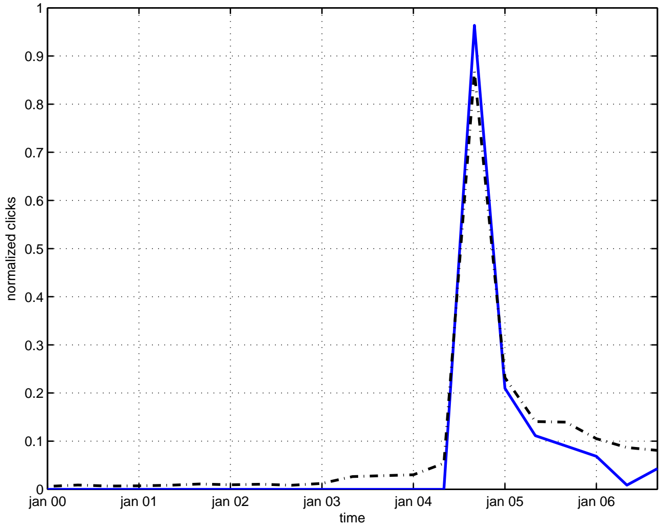
conformal thermodynamics
