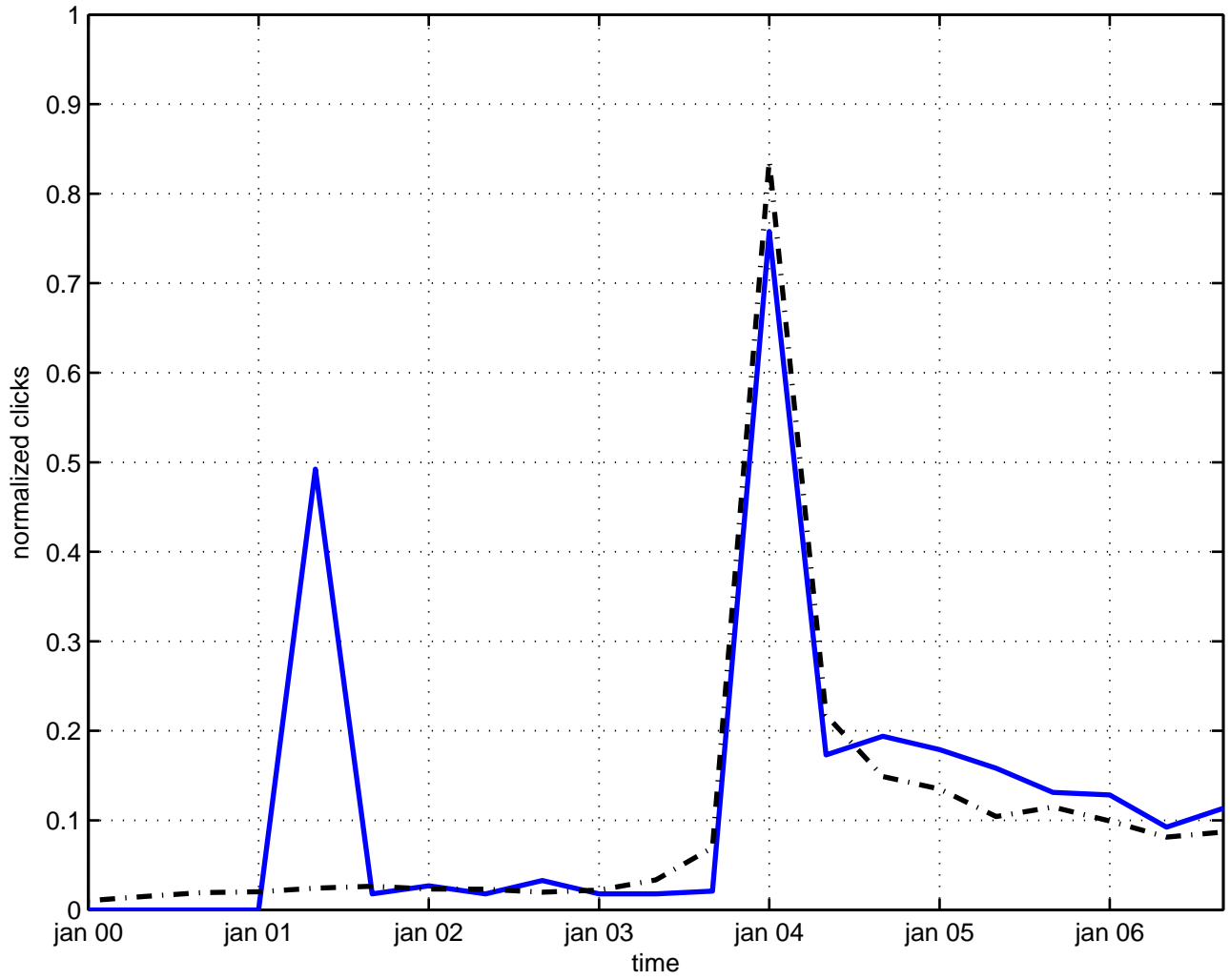
conformal supersymmetry
