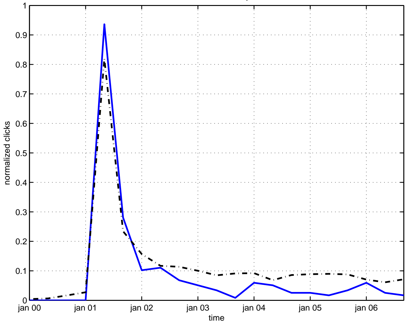
conformal stability
