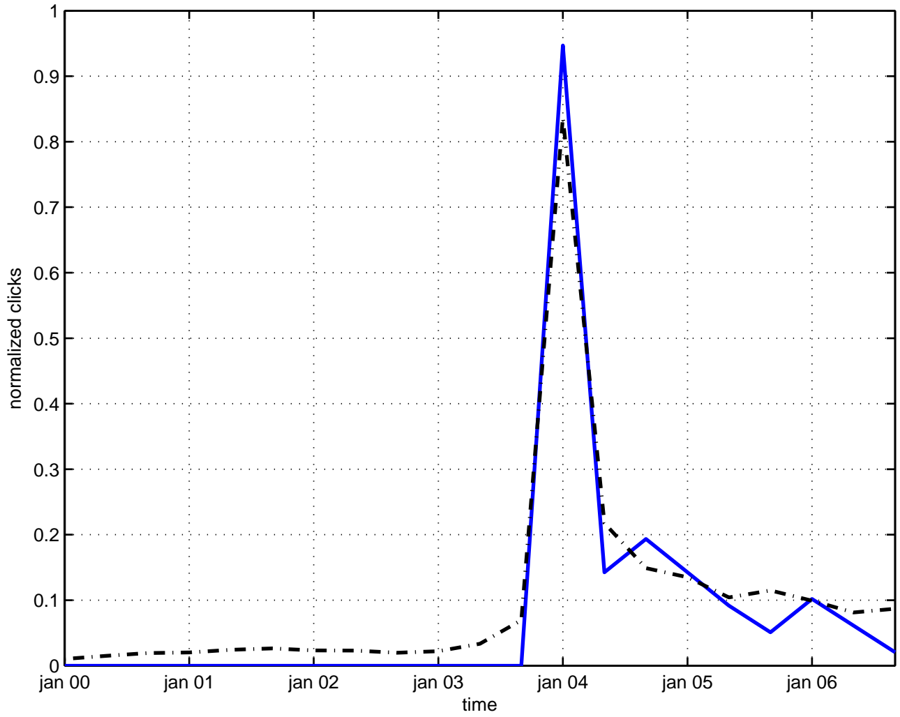
conformal scaling
