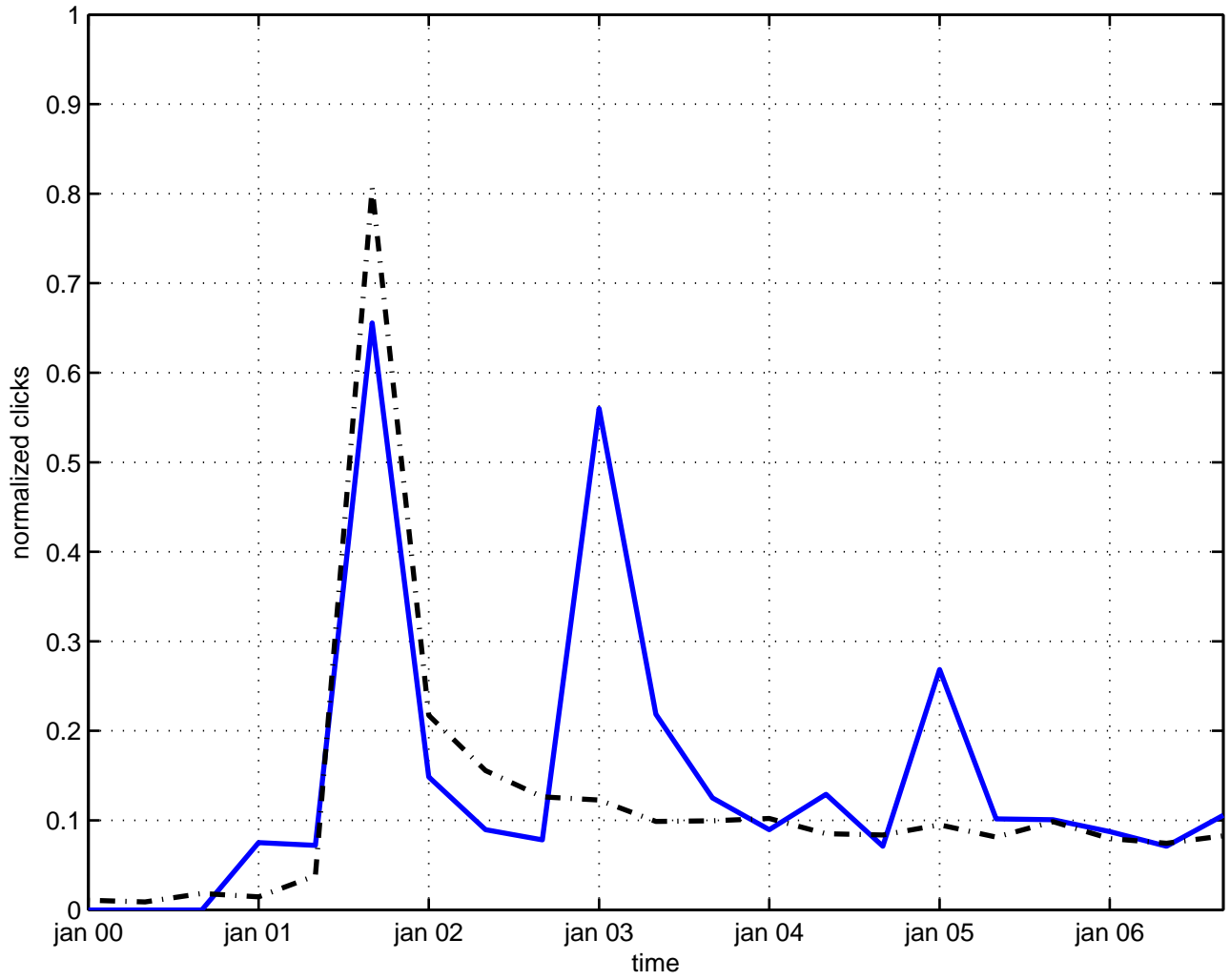
conformal operator
