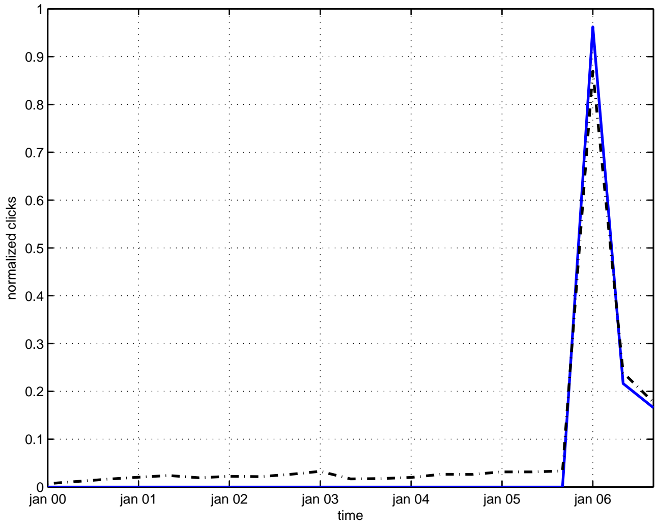
conformal interaction
