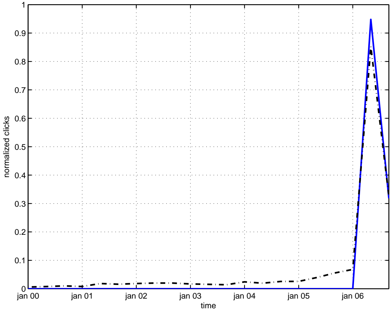
conformal holography
