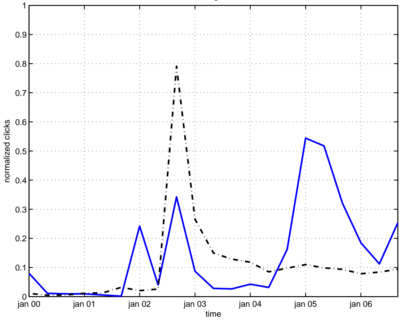
conformal gravitation
