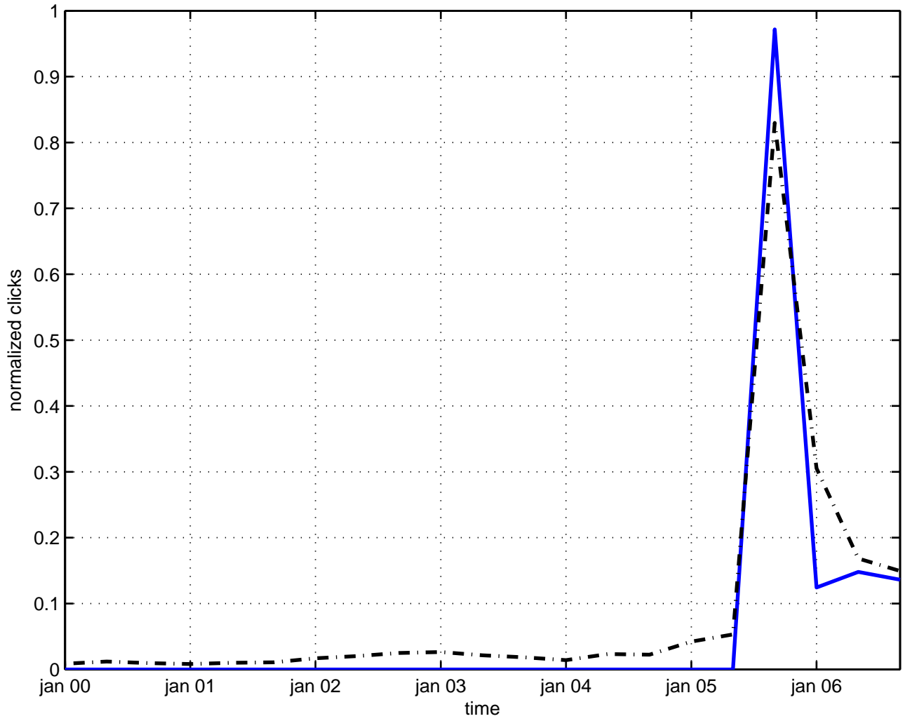
conformal geometry
