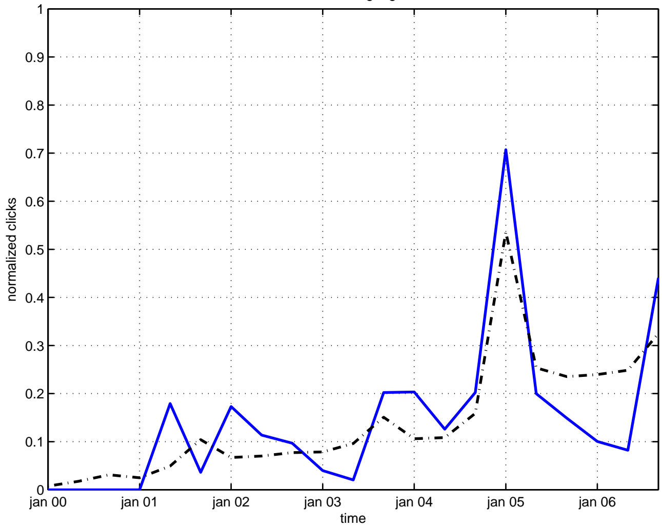
conformal gauge
