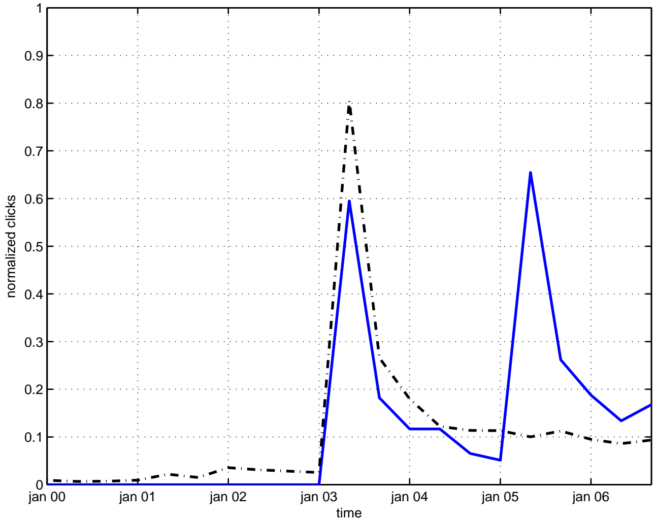
conformal gauge field theory
