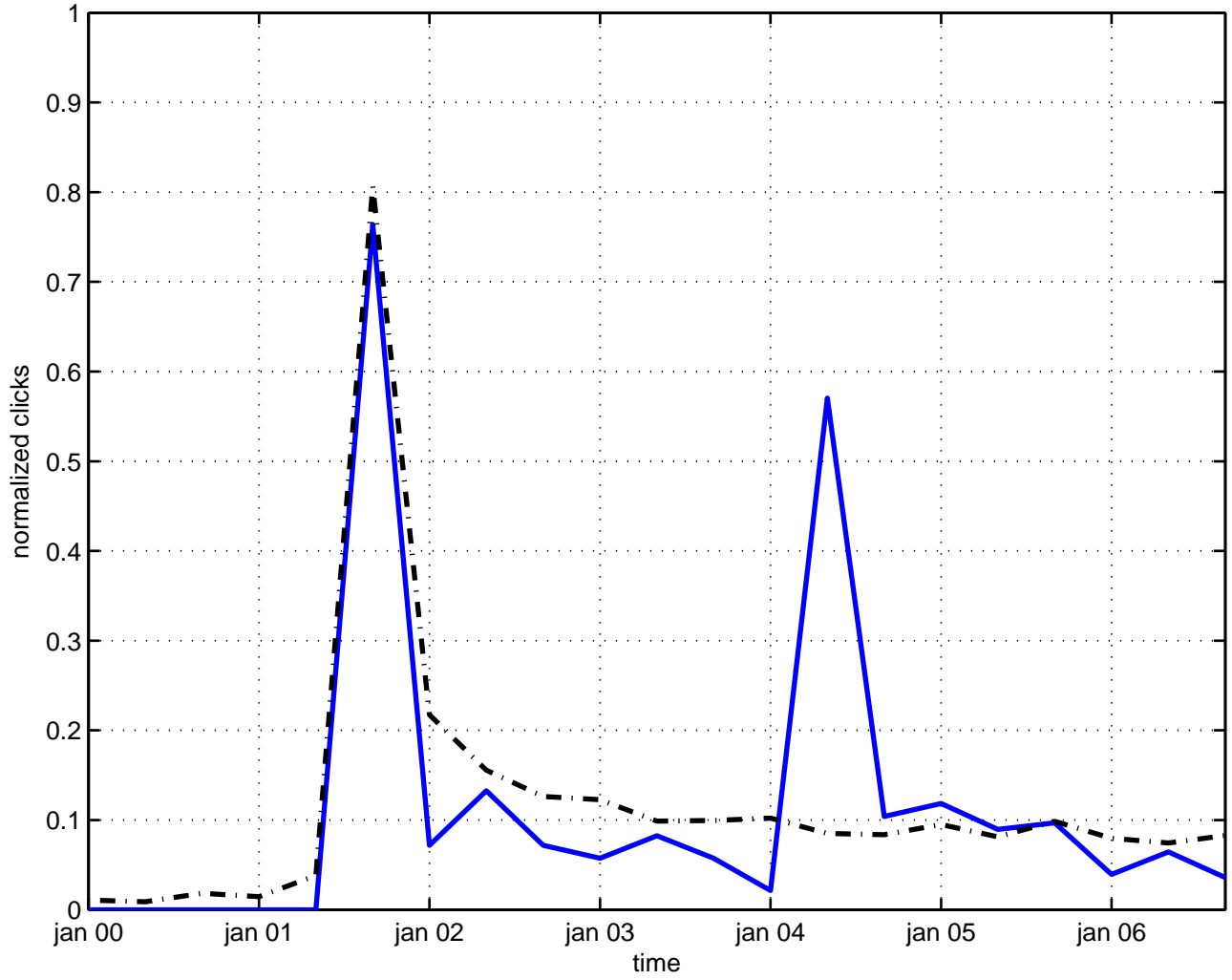
conformal energy
