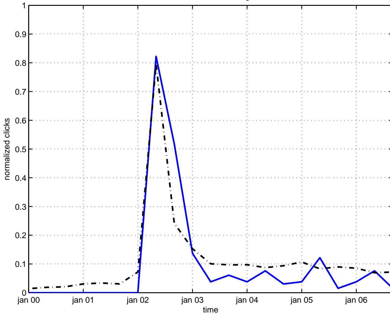
conformal embedding
