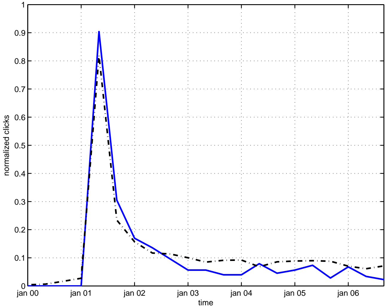
conformal correlation function
