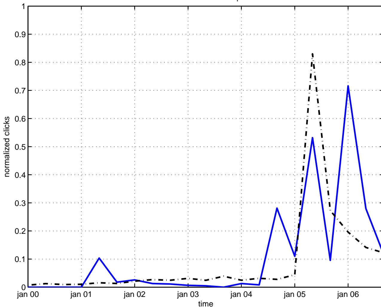
conformal bootstrap
