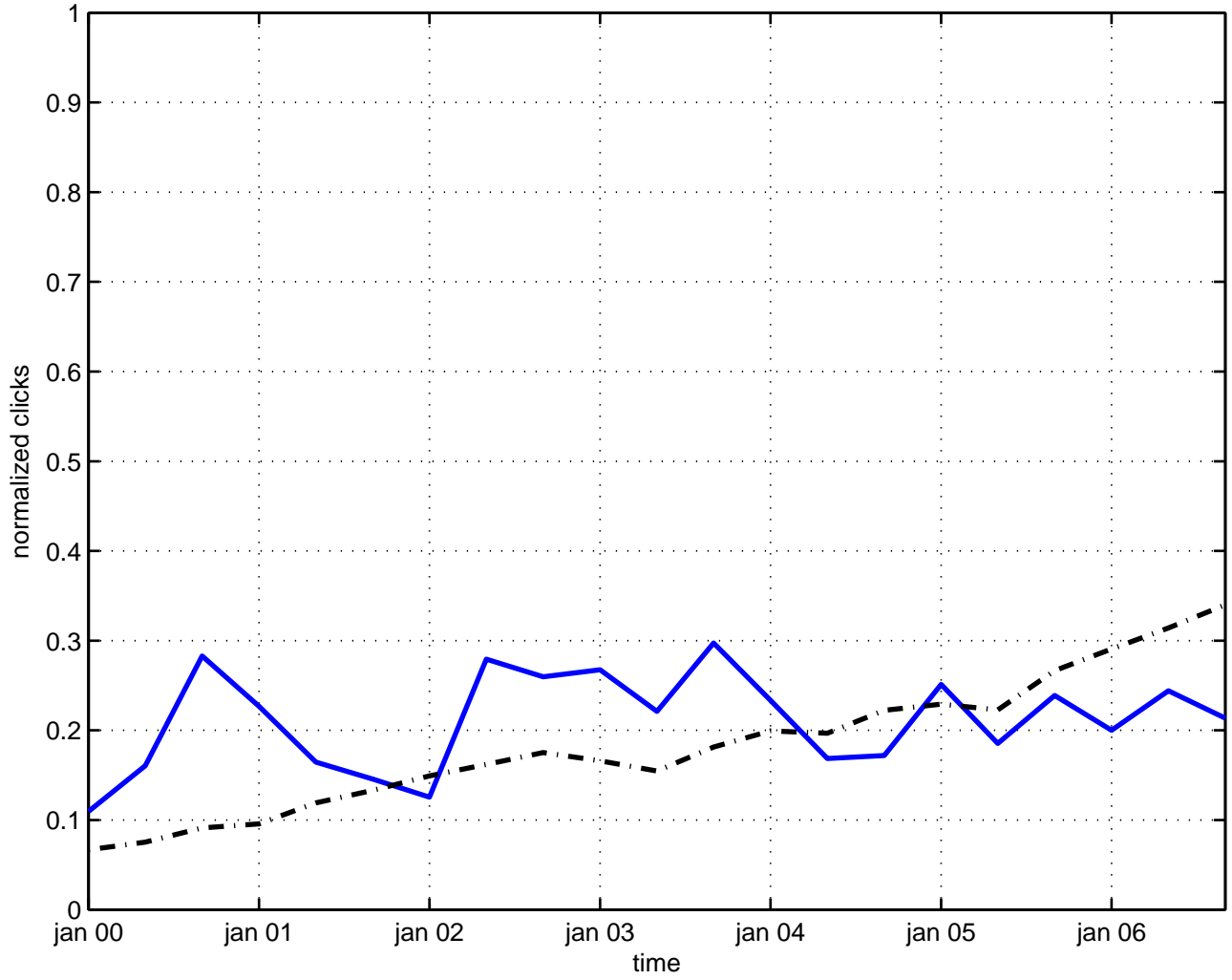
conformal anomaly
