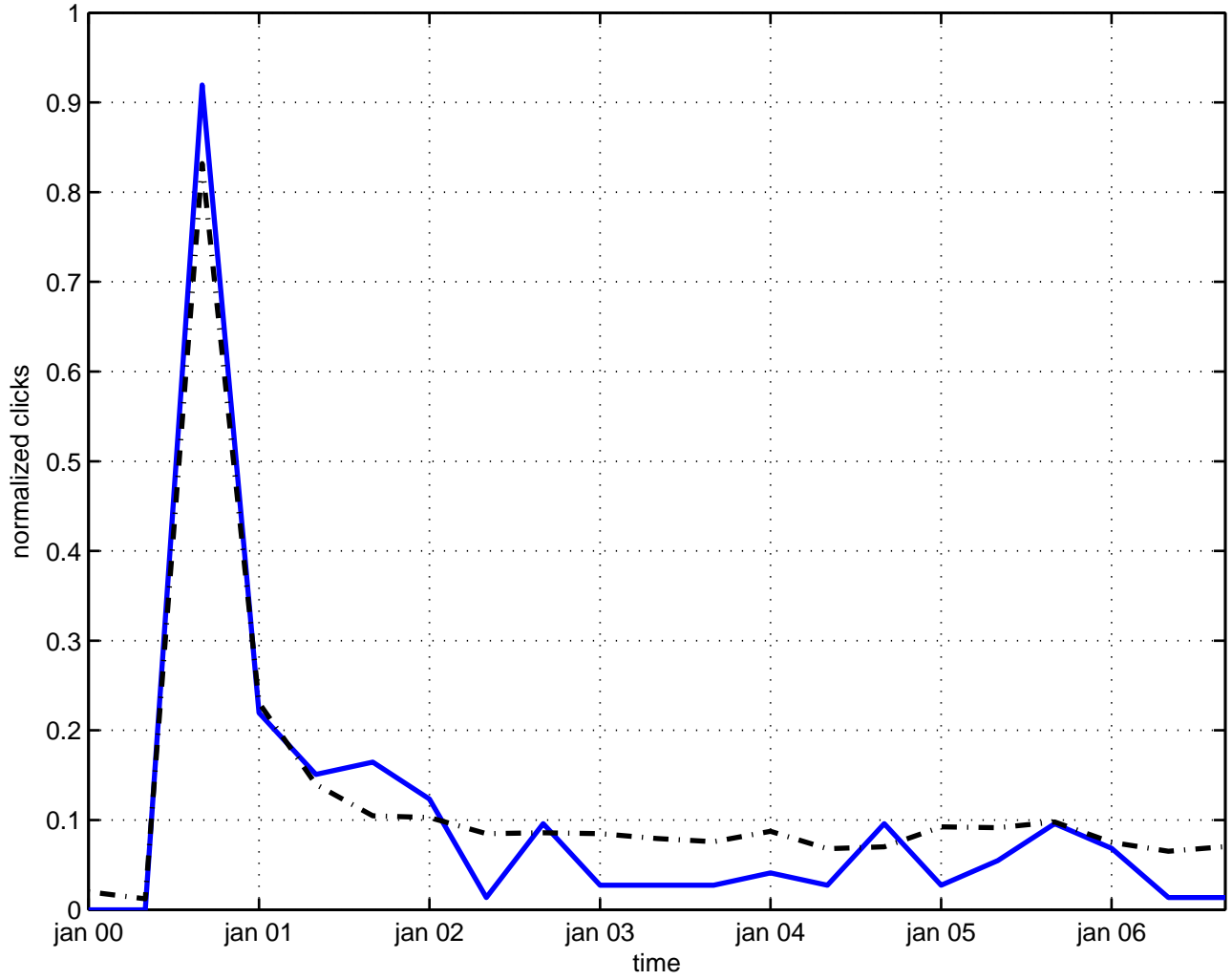
confinement plasma
