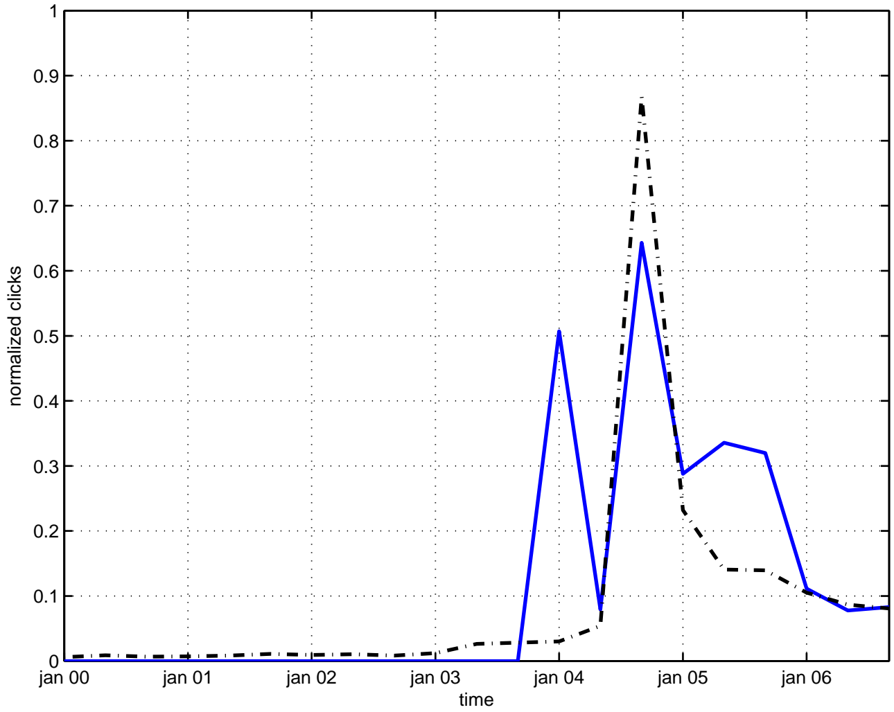
confinement gluon
