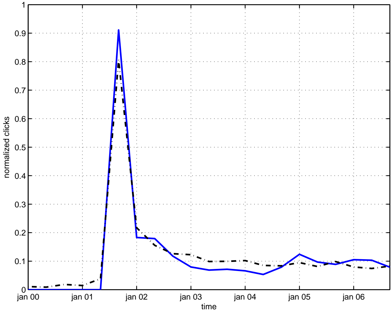
confinement gauge field theory
