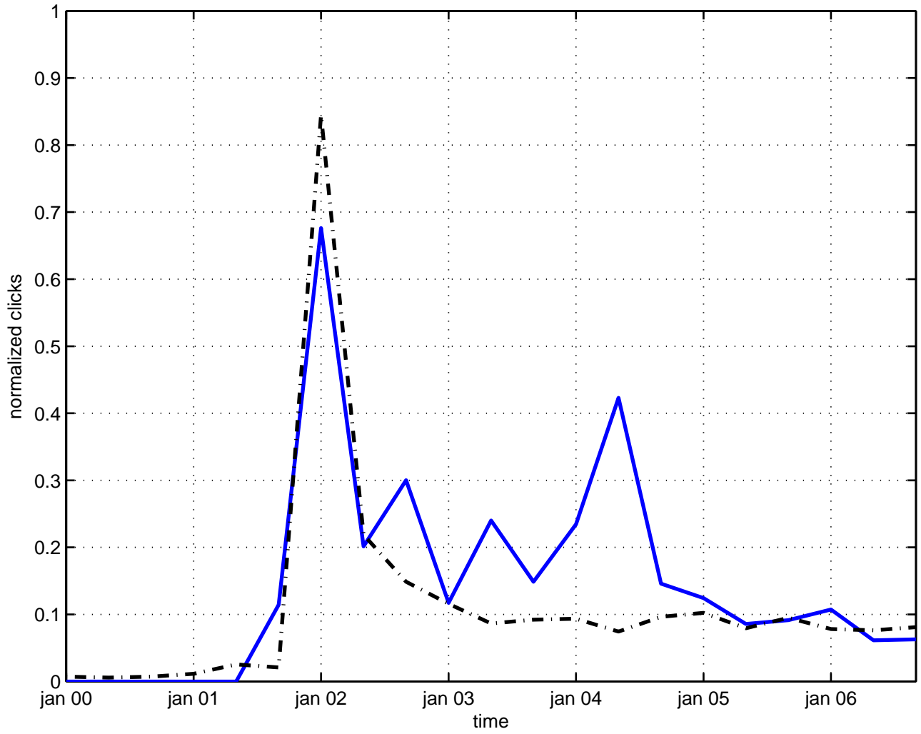
condensation vacuum state
