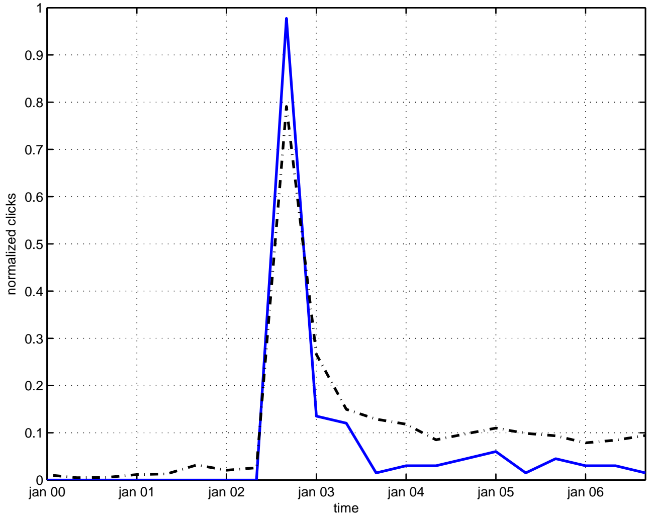
condensation quasiparticle
