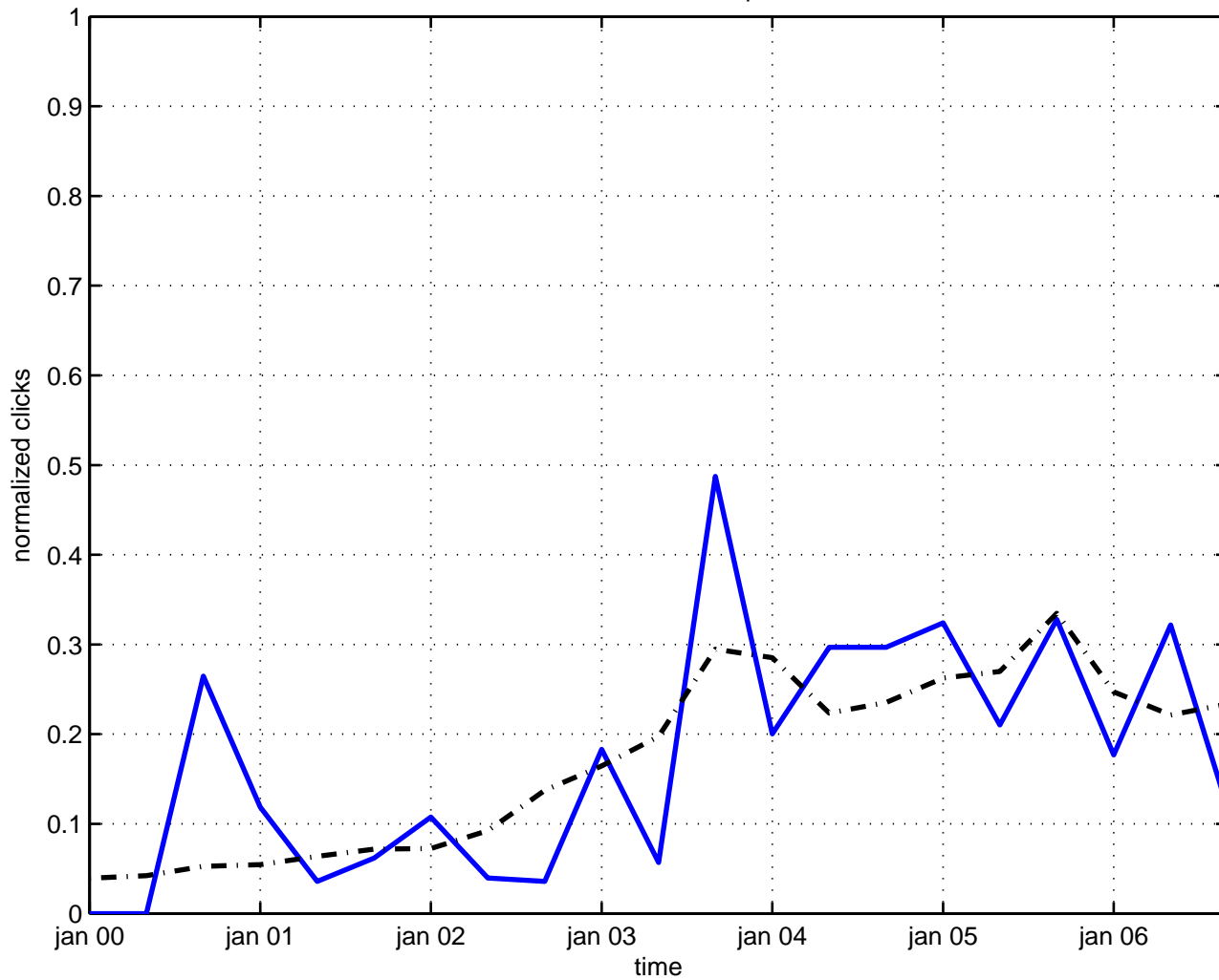
condensation monopole
