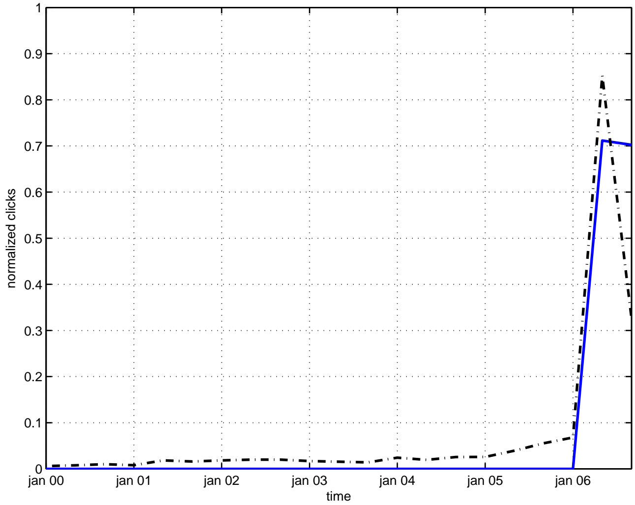
condensation higgs particle
