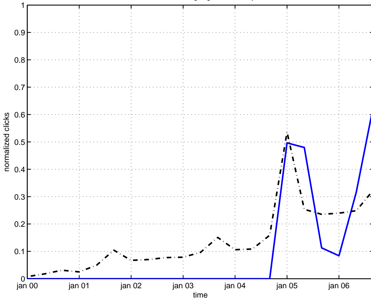
condensation gauge field theory
