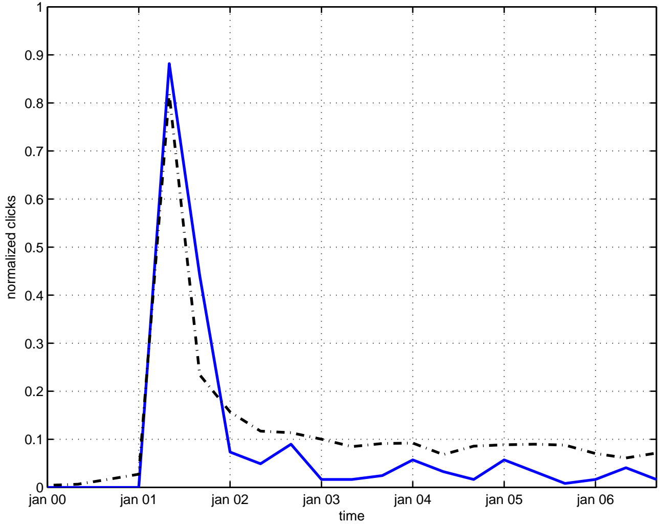
condensation f0(600)
