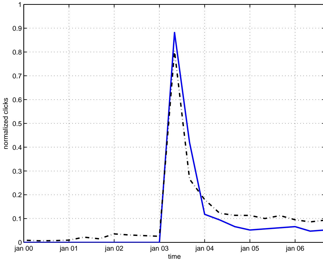
condensation born-infeld model
