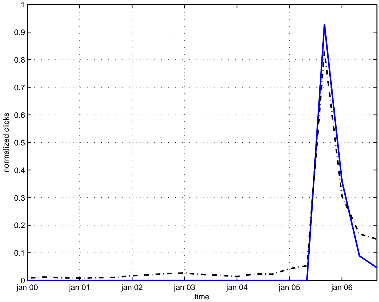
condensation black hole
