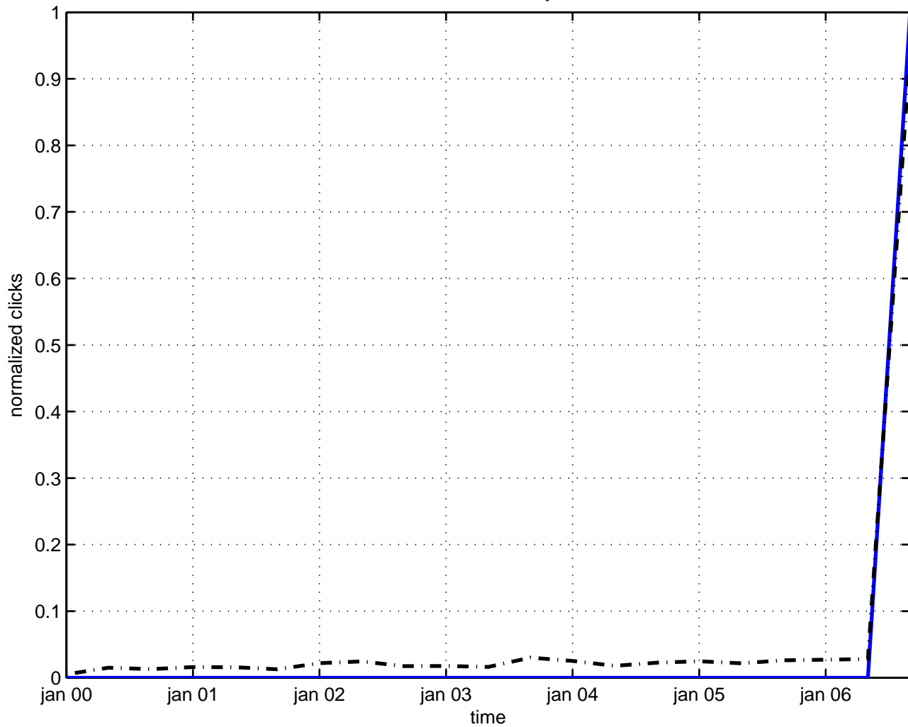
condensation baryon
