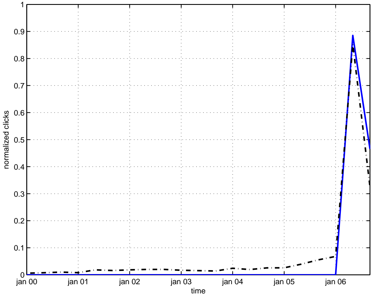
compton scattering photon hadron
