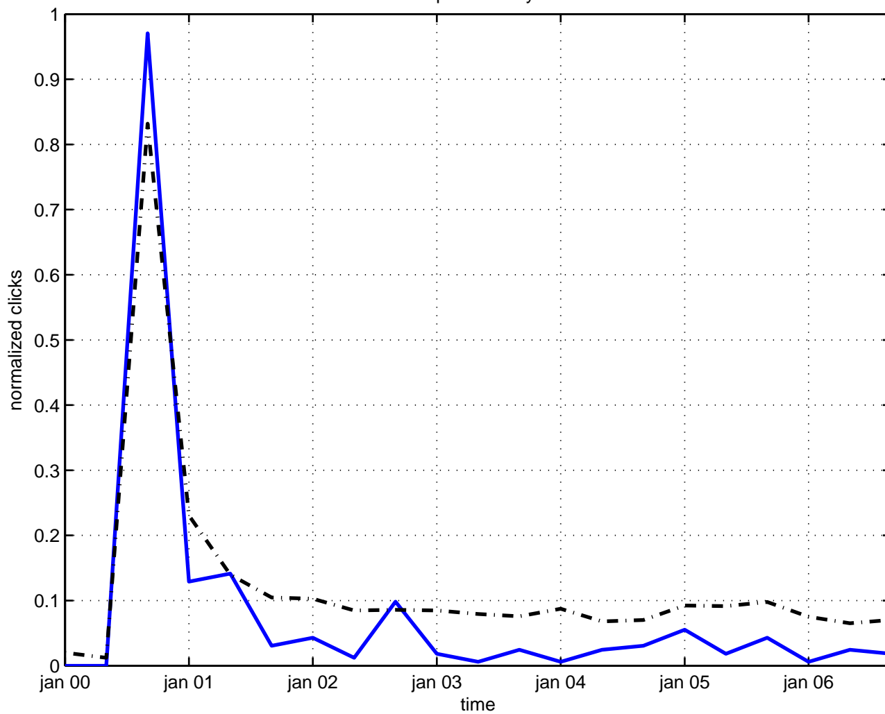
composite tachyon
