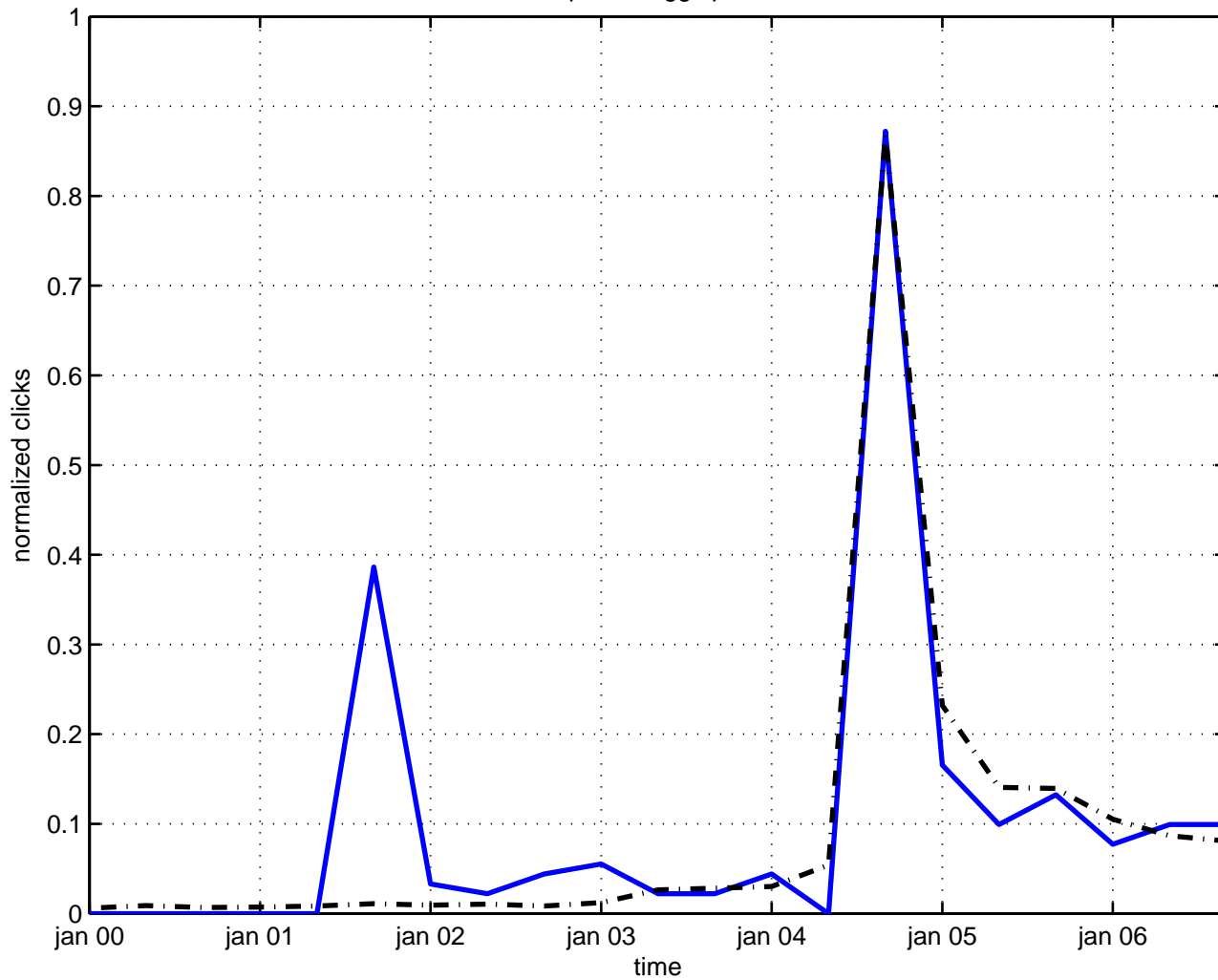
composite higgs particle
