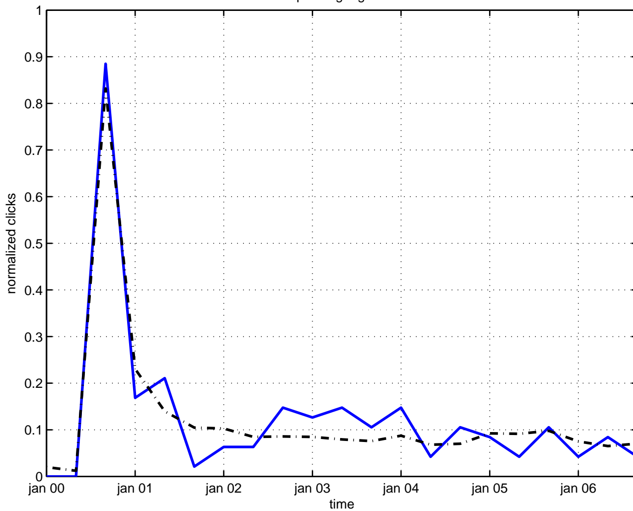
composite gauge boson
