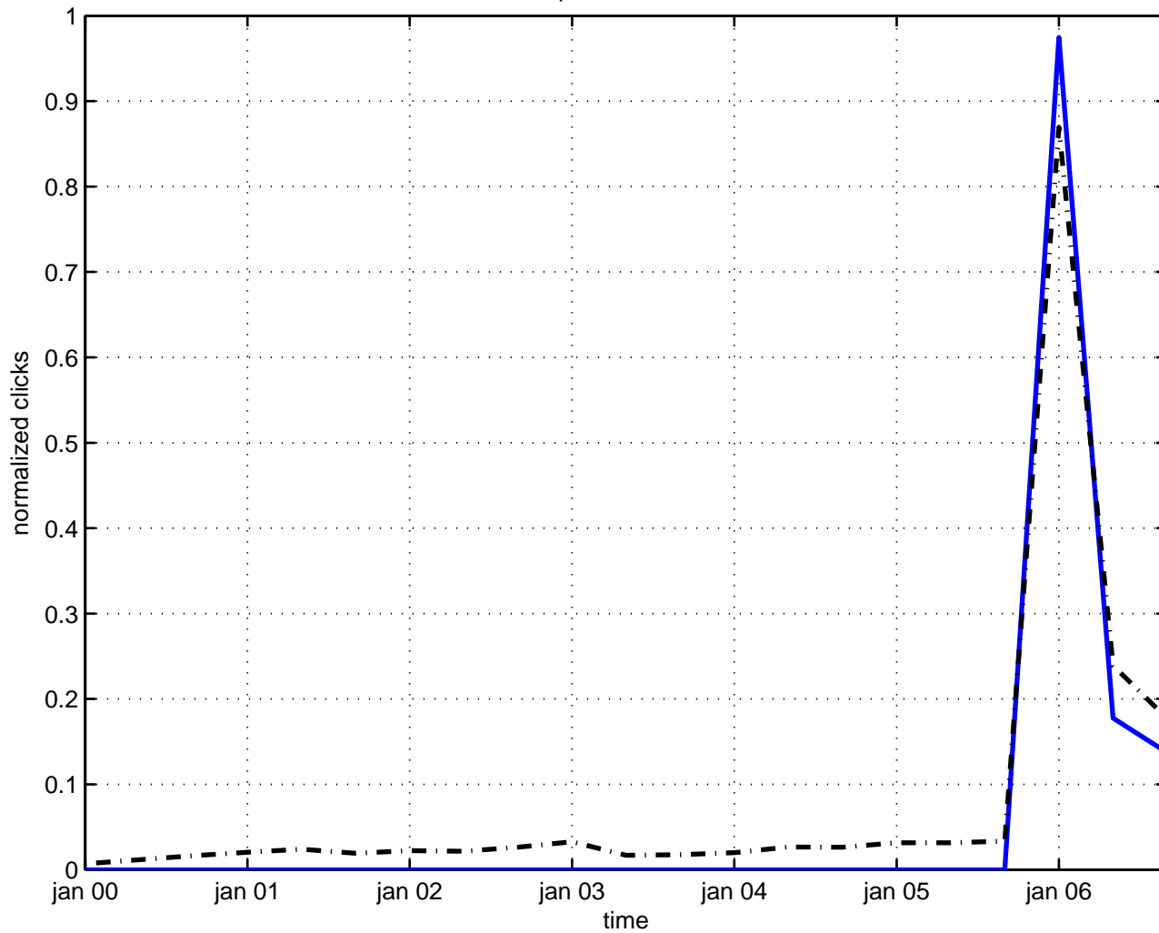
compactification time
