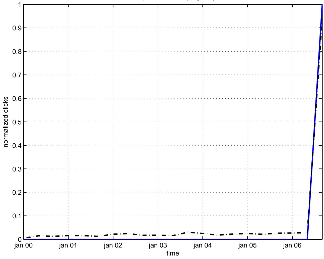
compactification supergravity
