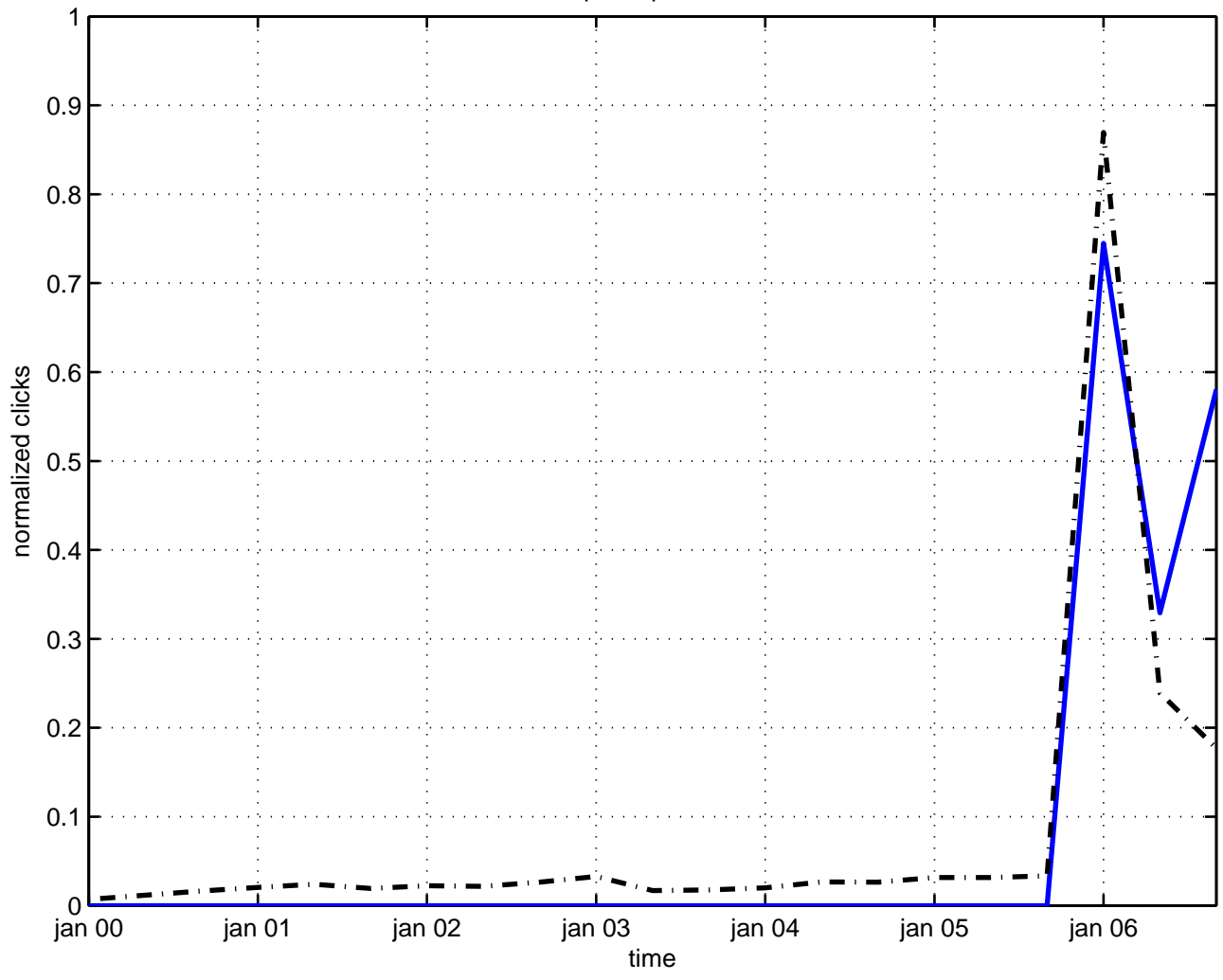
compact space-time
