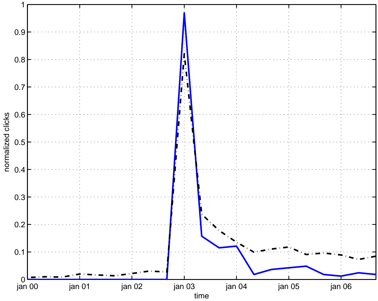
compact lattice field theory
