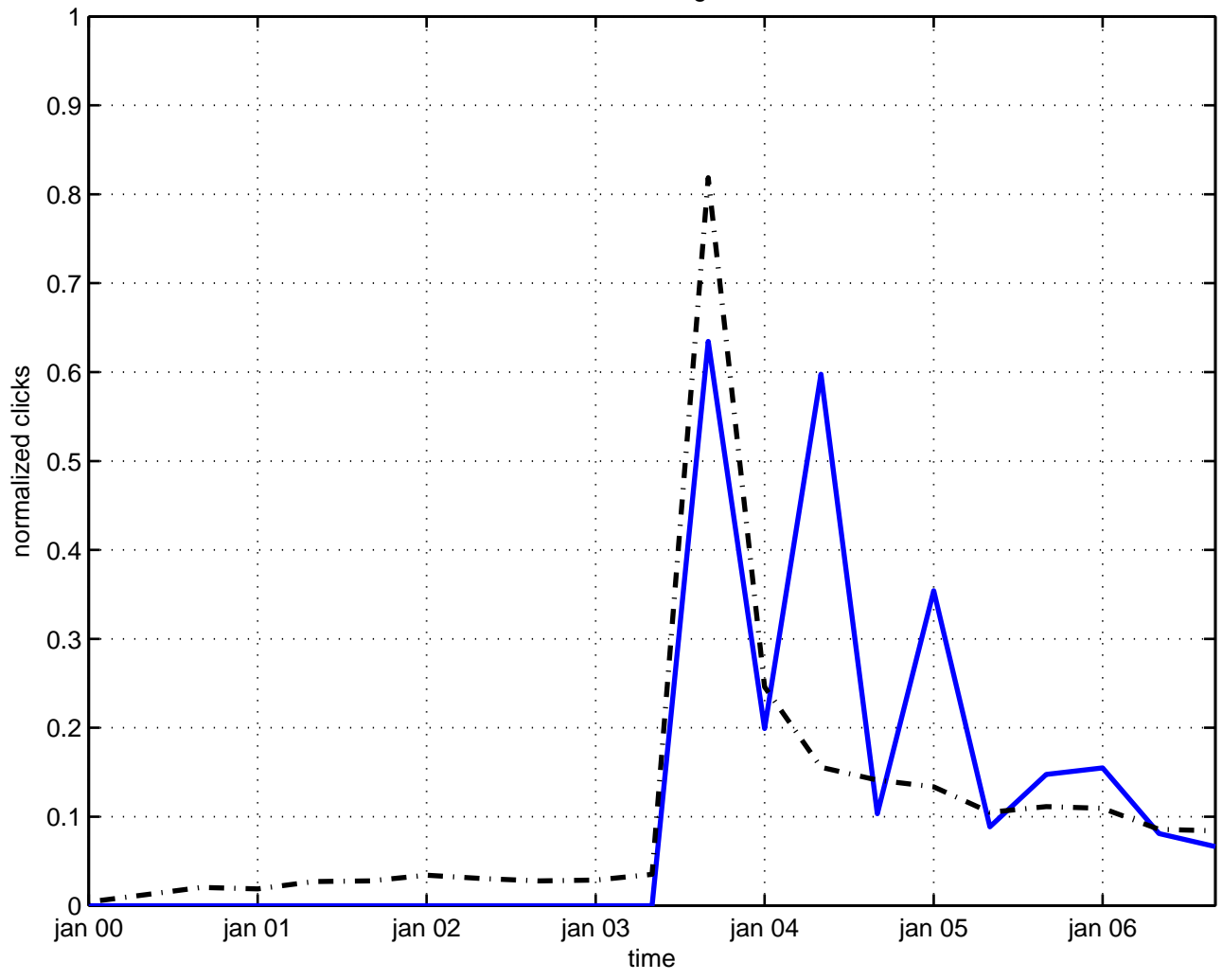
color charge
