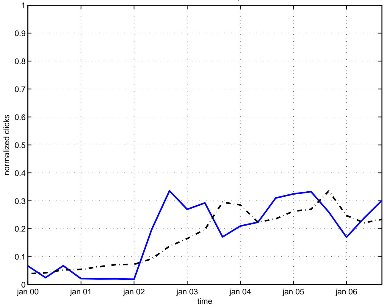
collective field theory
