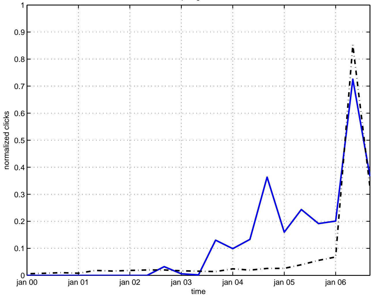
collapse gravitation
