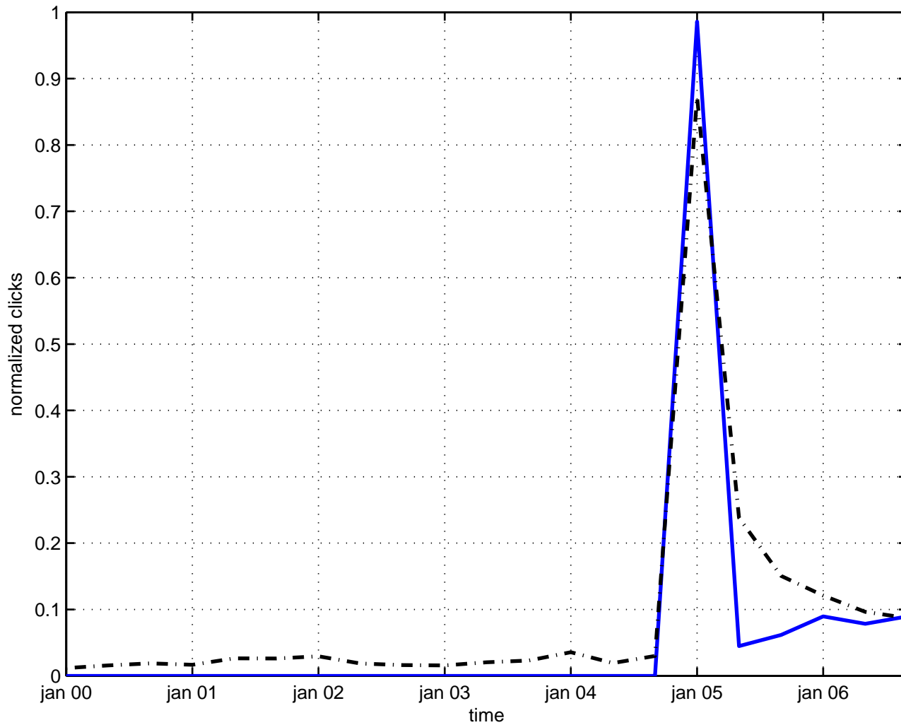
coherent state fermion
