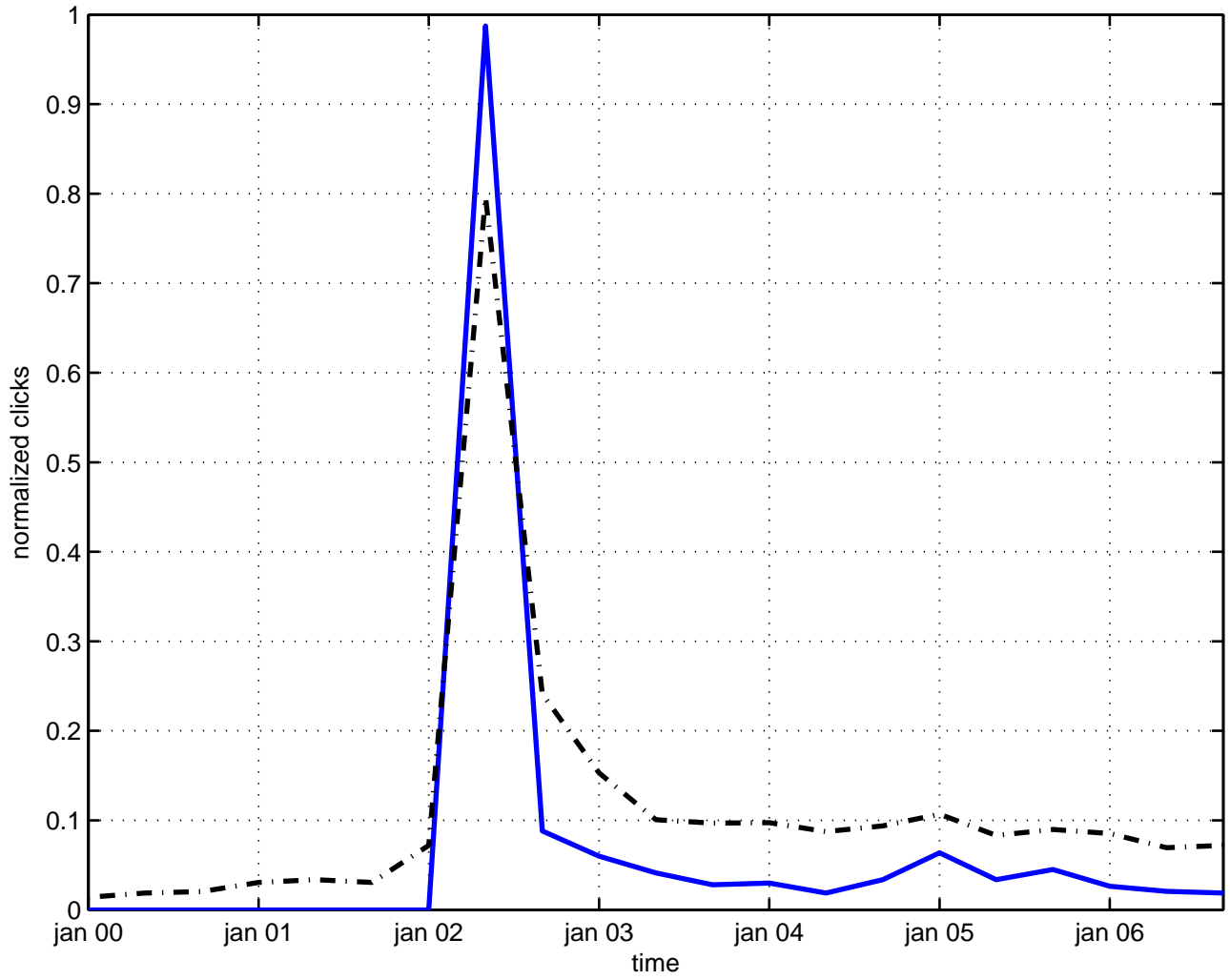
cluster gravitation
