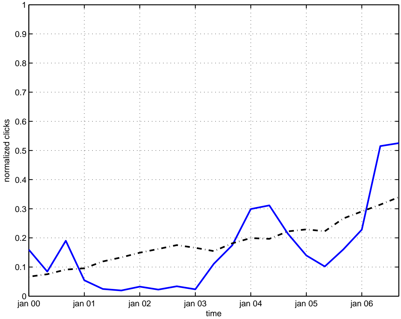
cluster expansion
