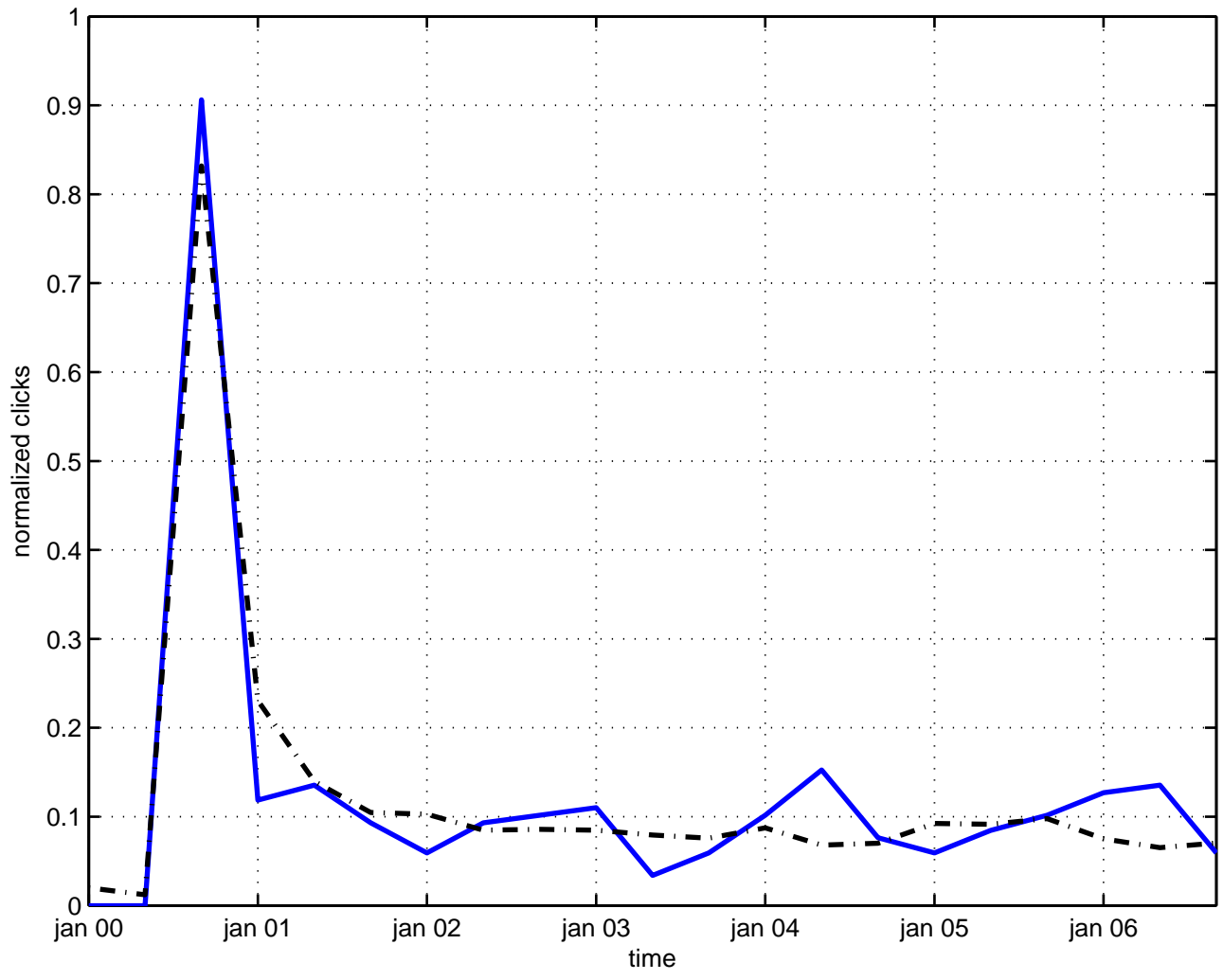
cluster electron
