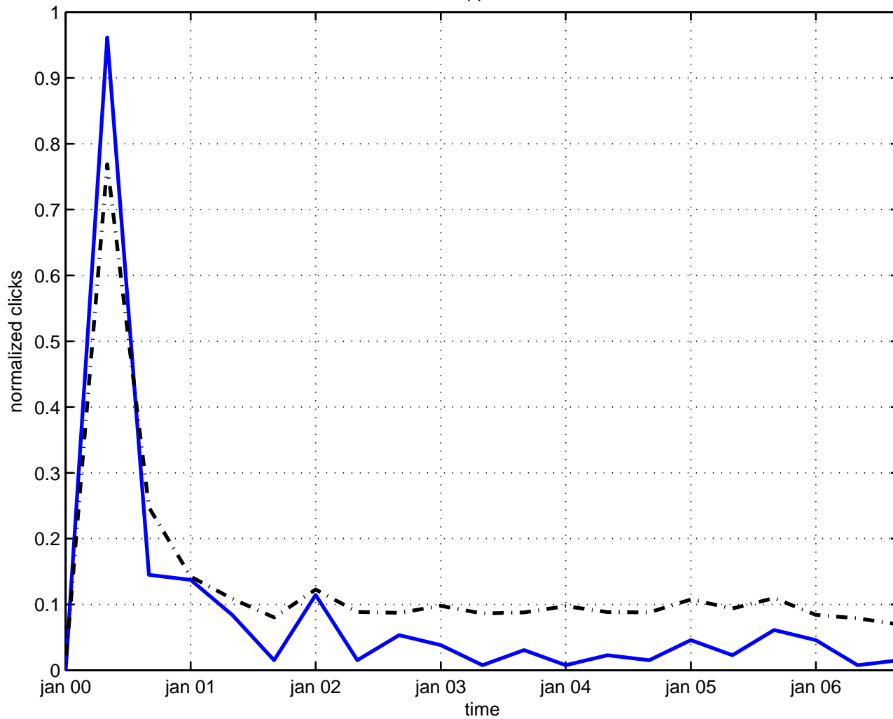
closure approximation
