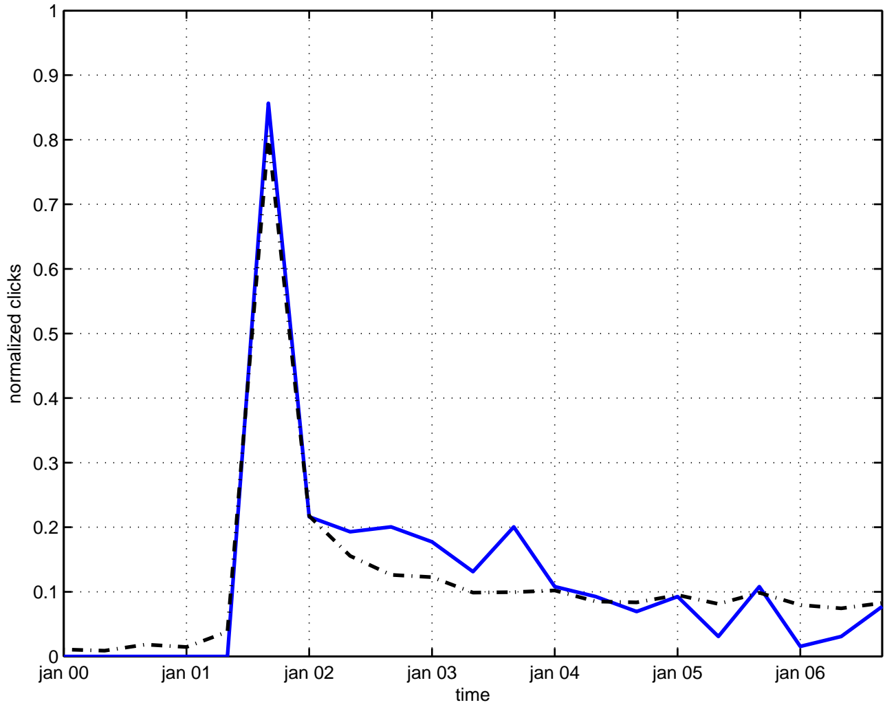
clifford spinor
