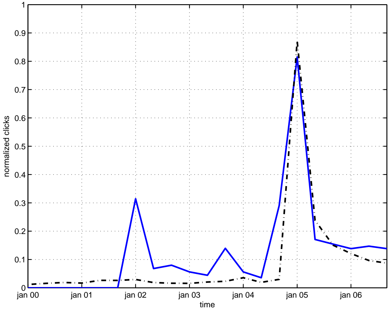
clifford space
